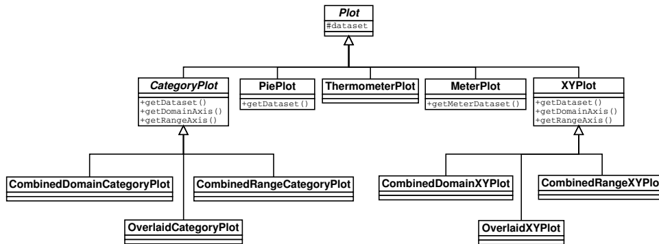
Figure 34.16: Plot classes
