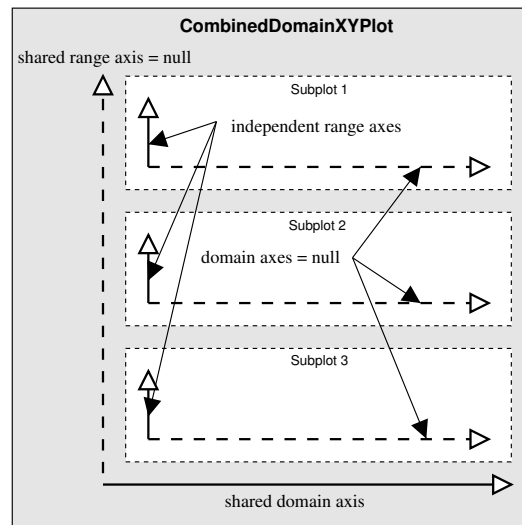
Figure 34.4: CombinedDomainXYPlot axes
