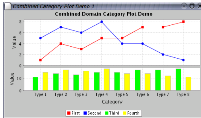
Figure 34.3: A CombinedDomainCategoryPlot
